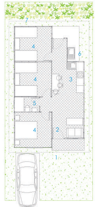
42M 2 HOUSE - expanded
