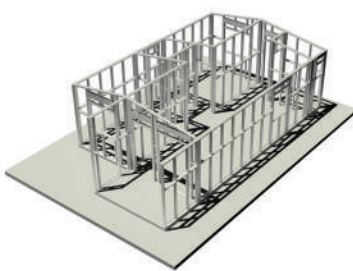
1. Foundation and studs
