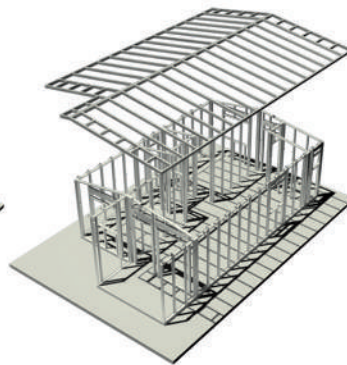
3. Union roof- studs
